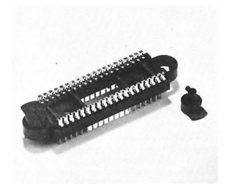
Figure 4. Since the contacts mate with both sides of the substrate, metallization can be on either, or both sides.
